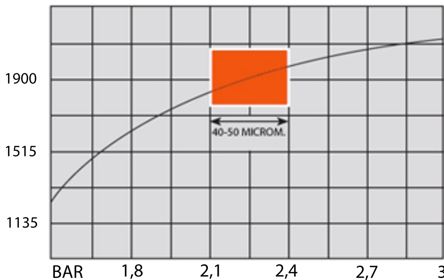
Liter/Minute 10" DESANDER CONE PERFORMANCE
